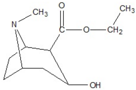
Ecgonine ethyl ester
